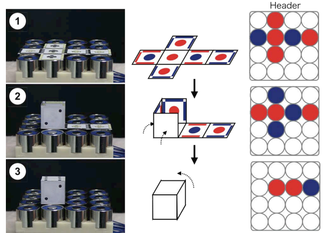
Figure 18. Electromagnet control with order of paper folding and magnetic pattern design.
